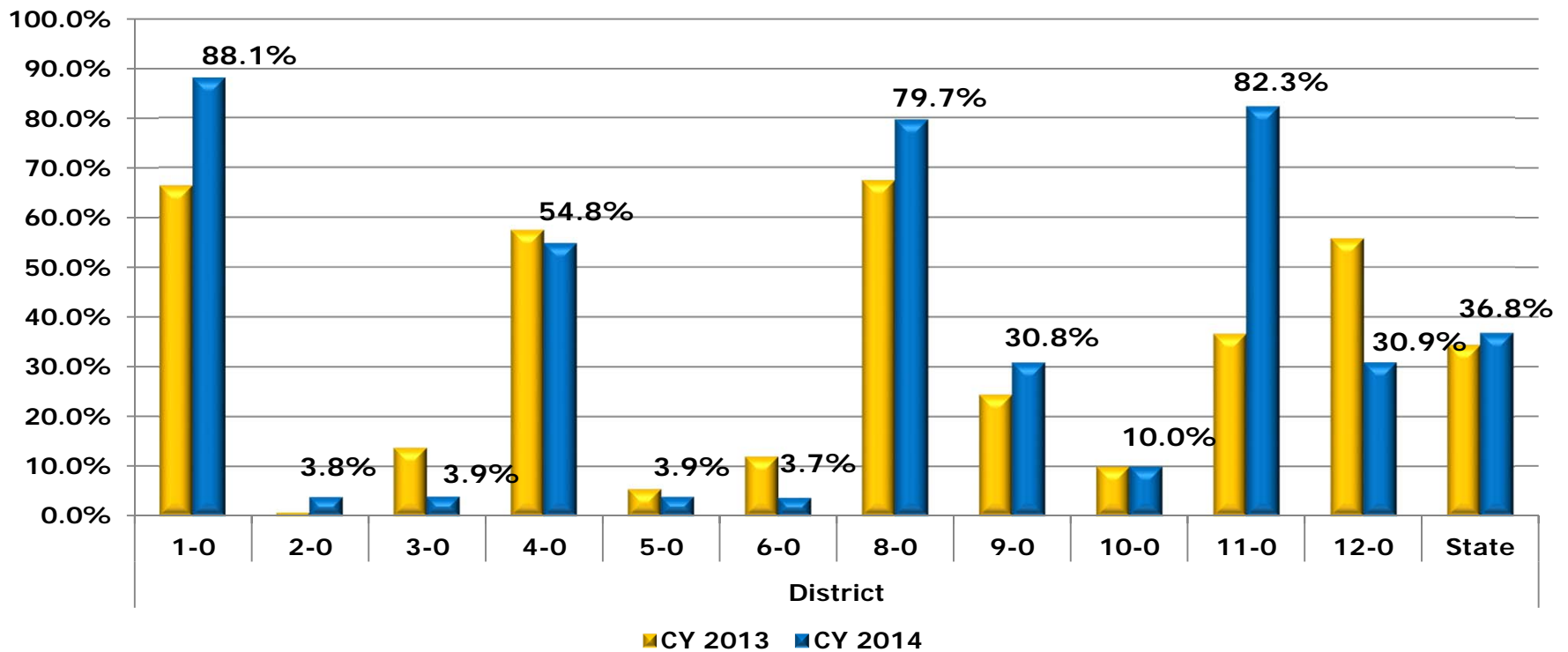
WMA Usage (% of Total Asphalt Tonnage)
